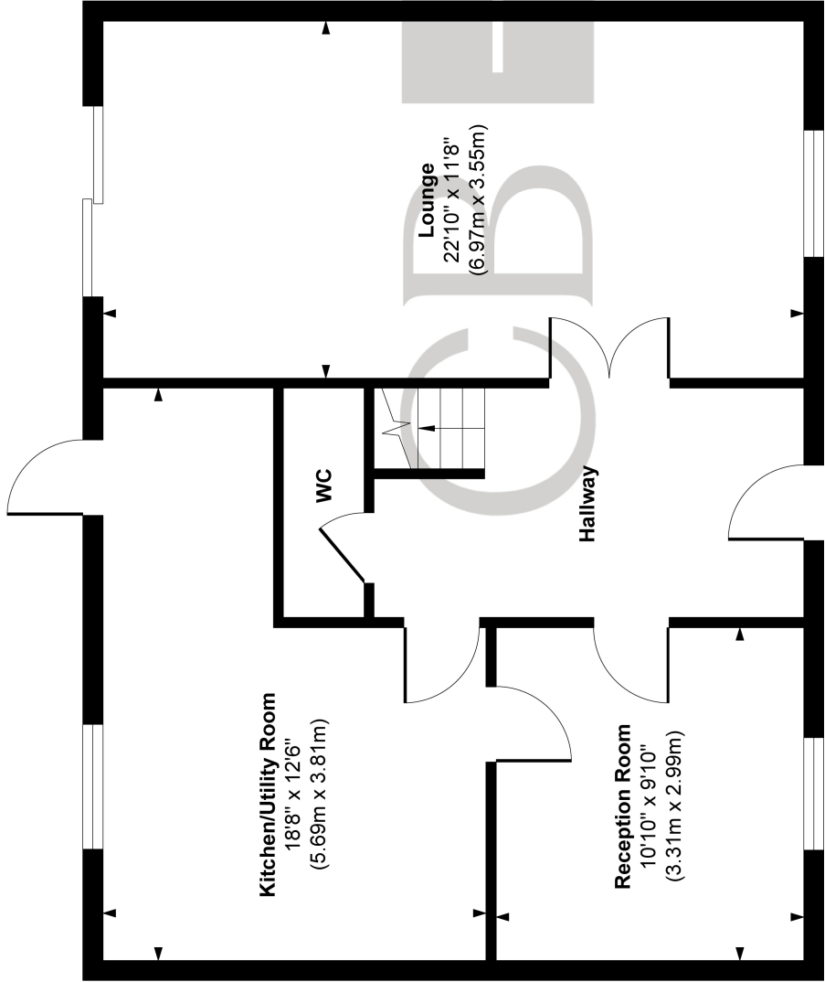
Ground Floor Approximate Floor Area 701 sq. ft (65.10 sq. m)
