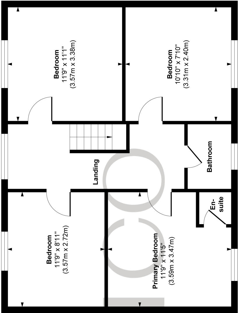
First Floor Approximate Floor Area 701 sq. ft (65.10 sq. m)
